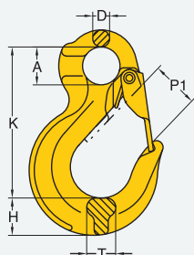
NS-EN 1677-2
